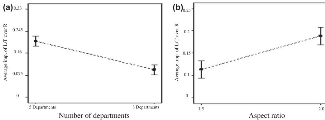
Figure 6. Significant main effects.
