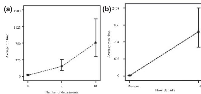
Figure 3. The effect of the number of departments and the flow density on the run time.
